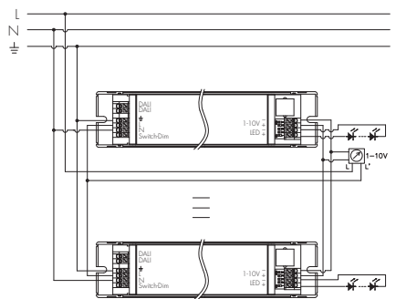
1-10V Wiring Diagram
