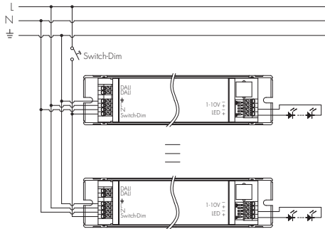
Switch-Dim Wiring Diagram
