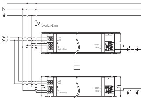
DALI + Switch-Dim Wiring Diagram
