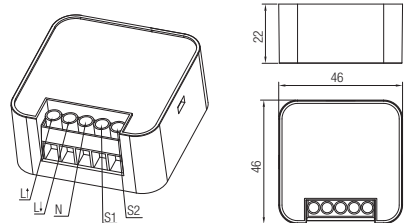
Typical Switch Box Mounting
