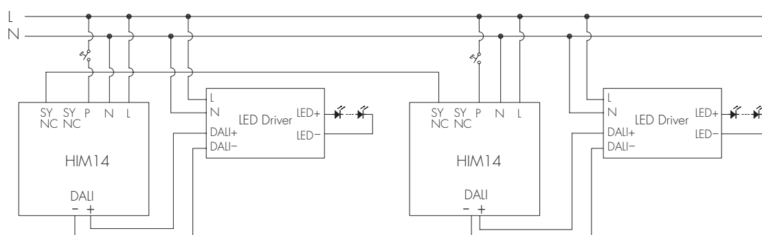
Wiring Diagram
